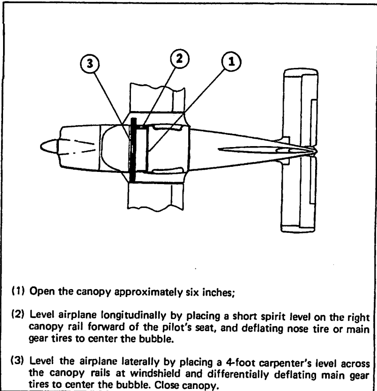
Figure 6-1. Airplane Leveling
