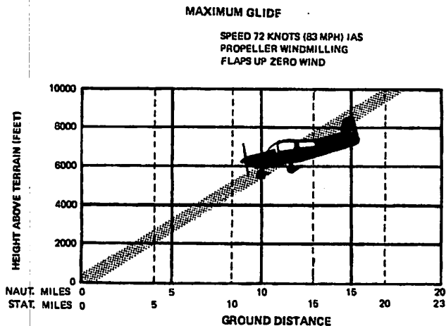
Figure 3.1 Maximum Glide
