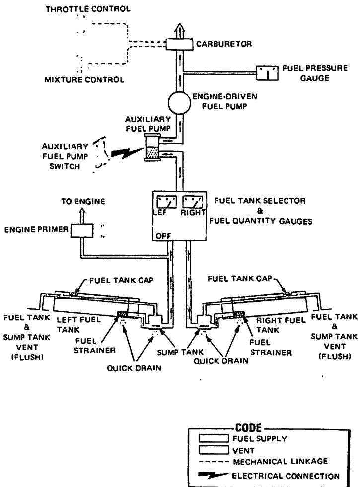
Figure 7-2 Fuel System
