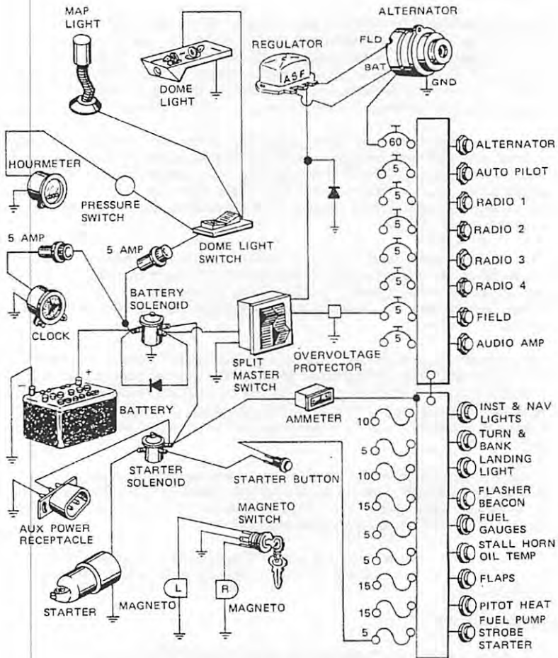
Figure 7-3, Electrical System
