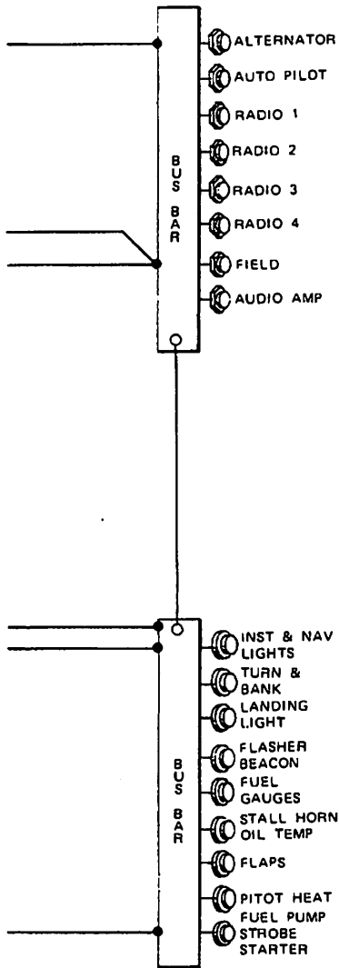
Figure 7-3 Electrical System (Sheet 2 of 2)
