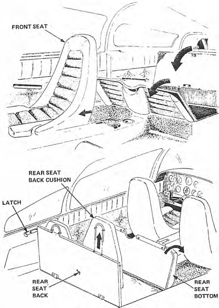
Figure 6-6. Rear Seat Stowage
