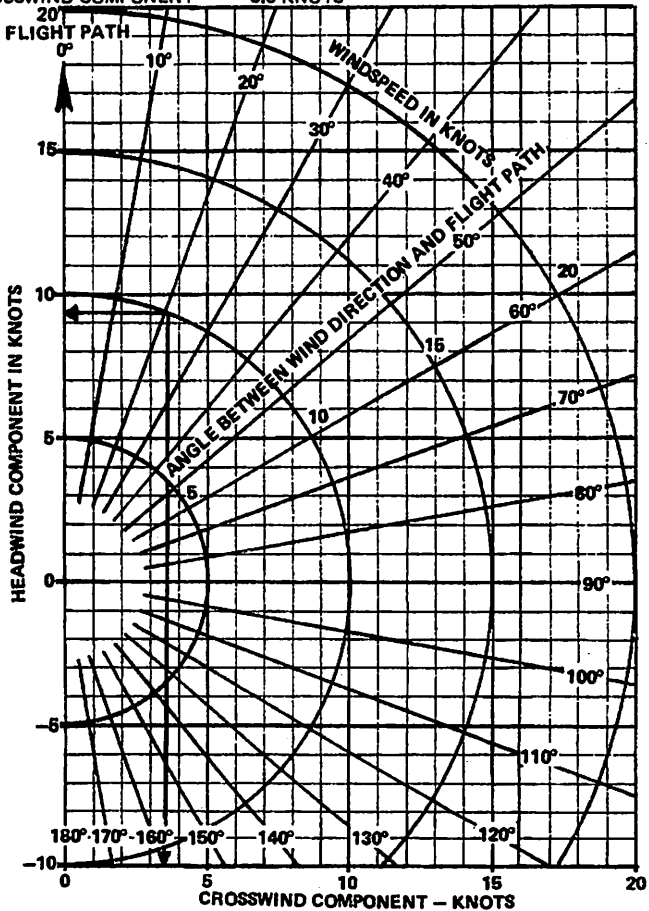
Figure 5-6. Crosswind Component Chart
