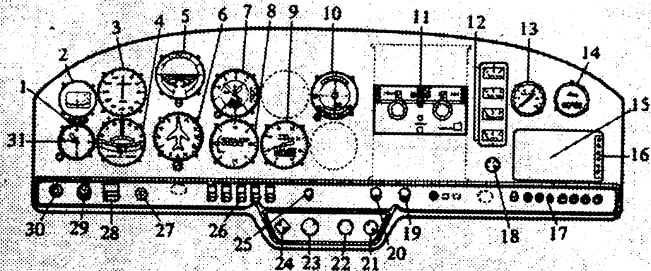
Figure 6. Yankee instrument panel diagram.
